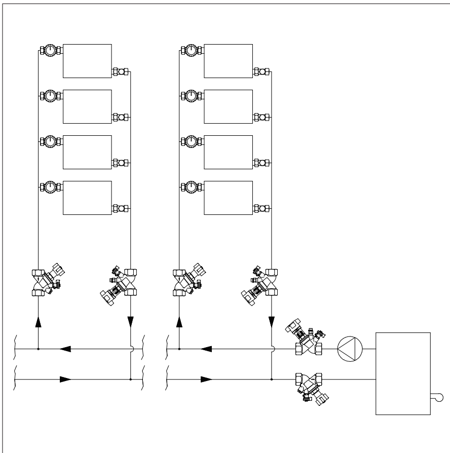
Example: Scheme of a two pipe heating system which has to be regulated to a pre-calculated design point by use of double regulating and commissioning valves.
