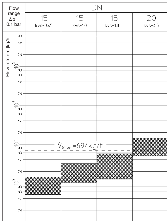
Regulating valve "Cocon 2TZ" with integrated metering station
