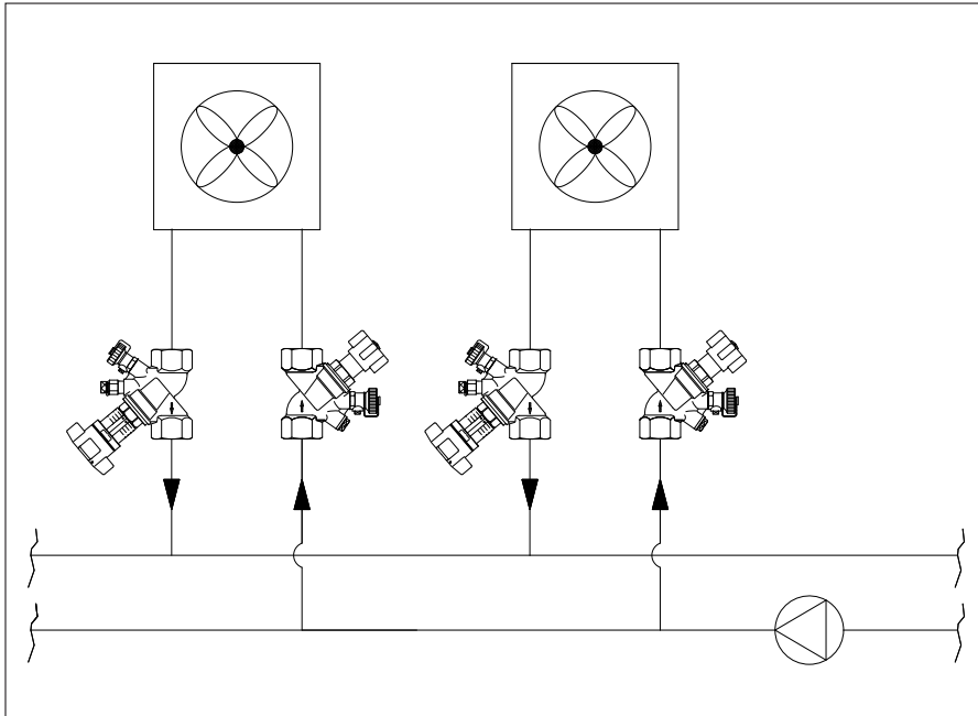
Example: Scheme of an air heating installation in which the flow rate is almost constant. Preset double regulating and commissioning valves provide a static hydronic balancing.
