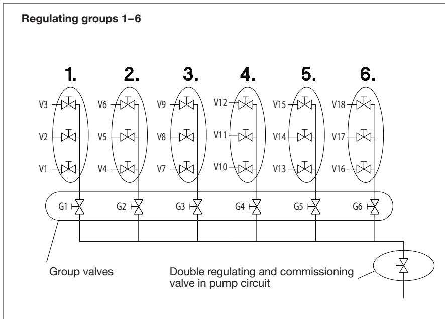
Example: OV-Balance method
