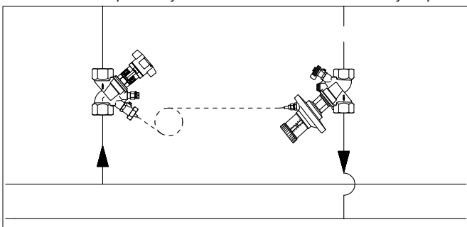
Example: Differential pressure regulation with flow limitation in installations with non-presettable thermostatic radiator valves.
