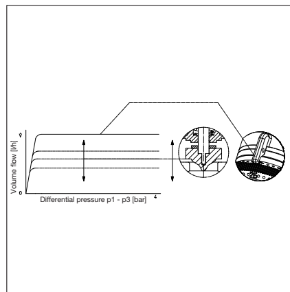
Volume flow characteristic line for different presettings
