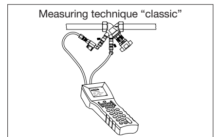
Regulation at double regulating and commissioning valve "Hydrocontrol VTR"
