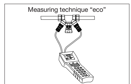
Regulation at double regulating and commissioning valve "Hycoccon VTZ"
