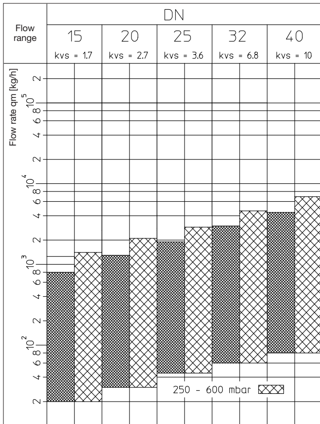
Flow ranges of the differential pressure regulator “Hycococon DTZ” for adjustable differential pressures in the circuits 50–300 mbar or 250–600 mbar
