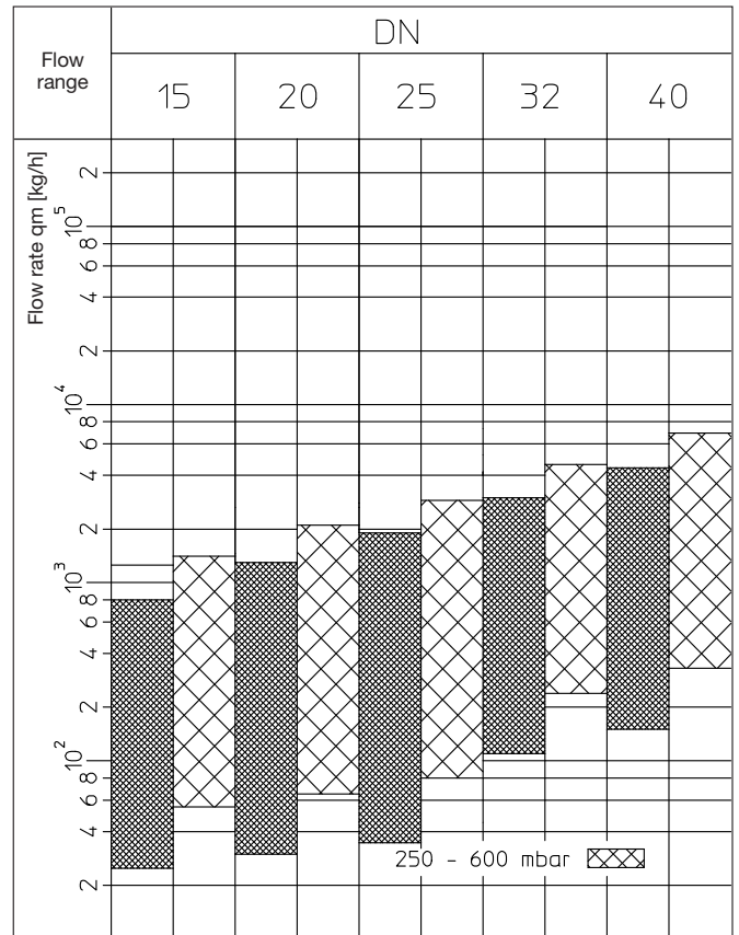
Flow ranges of the differential pressure regulator “Hycocon DTZ” for adjustable differential pressures in the circuits 50–300 mbar or 250–600 mbar and additional flow limitation at the double regulating and commissioning valve “Hycocon VTZ”
