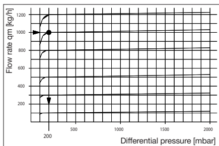
Volume flow characteristic line for different presettings
