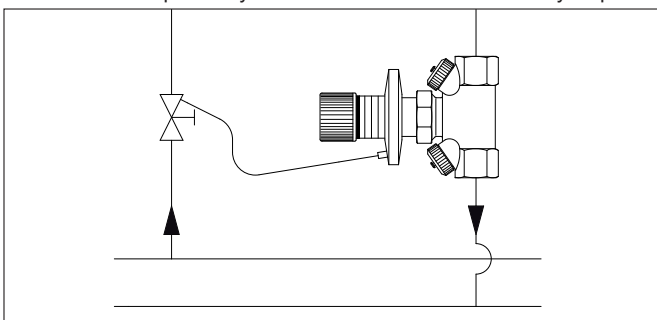
Example: Differential pressure regulation in installations with presettable thermostatic radiator valves (circuits with low to medium flow rate).
