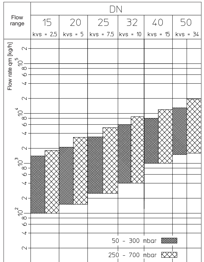
Flow ranges of the differential pressure regulator “Hydromat DTR” for adjustable differential pressures in the circuits 50–300 mbar or 250–700 mbar
