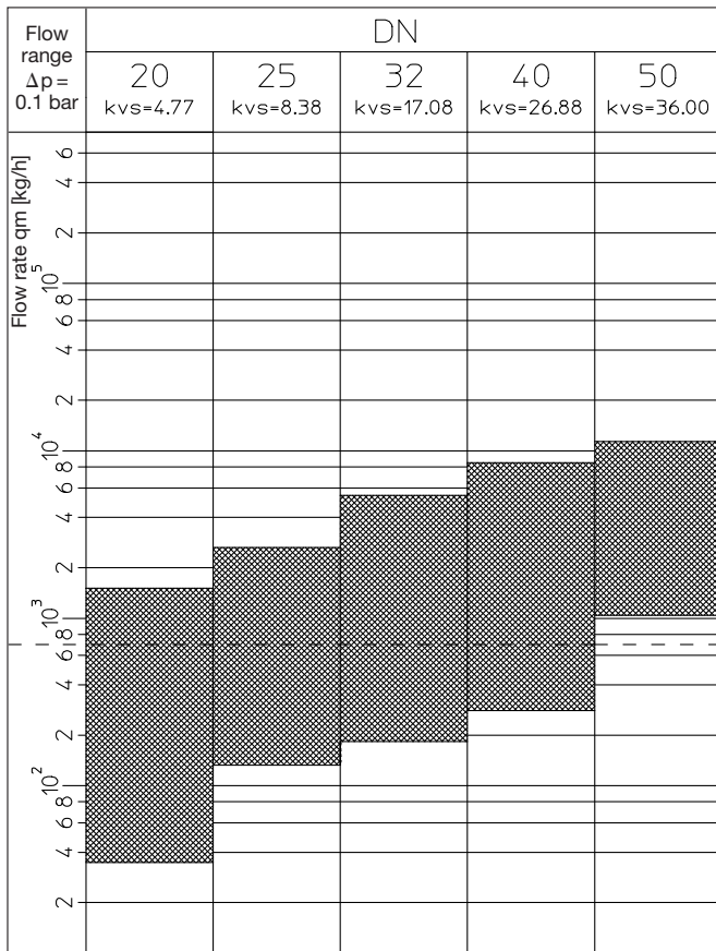
“Hydrocontrol VFC”
